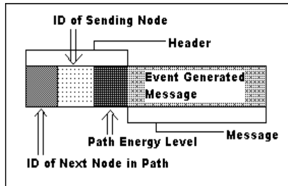
Figure 1: Packet structure
