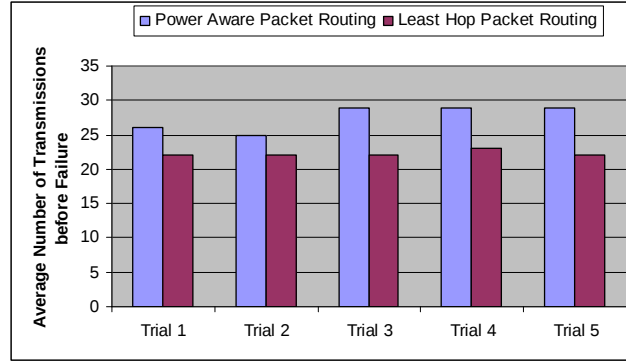
Figure 9: Large network, base-node placed in corner
