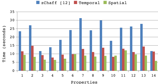
Fig. 5. Test Generation result for MIPS processor
